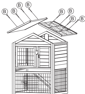
Step5: Secure roof
